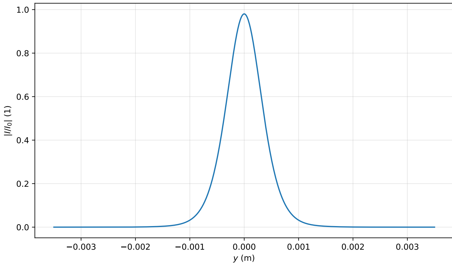
Intensity profile I(x=0, y, z=2.468)/I_0 , \text{Pin}=0.7\text{Pcr} , artificial time
